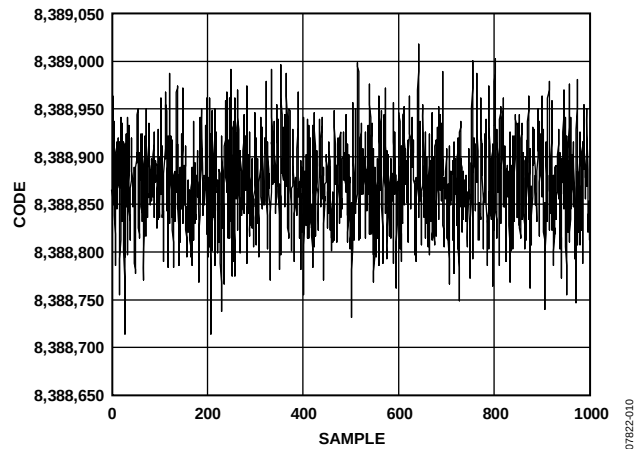
Figure 10. Noise ( V_{REF} = AV_{DD} = 5\text{ V} , Output Data Rate = 2400 Hz, Gain = 128, Chop Disabled, Sinc 4 Filter)
