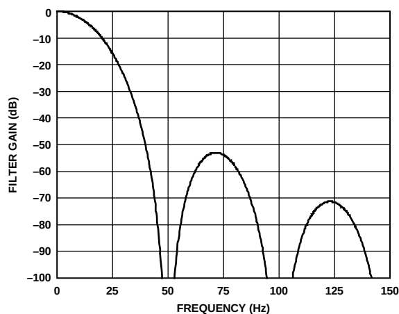
Figure 19. \text{Sinc}^4 Filter Response (50 Hz Output Data Rate)
