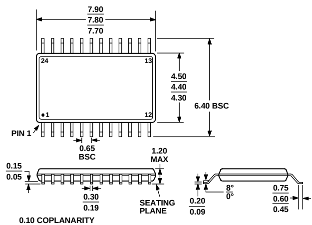
Figure 33. 24-Lead Thin Shrink Small Outline Package [TSSOP] (RU-24) Dimensions shown in millimeters
