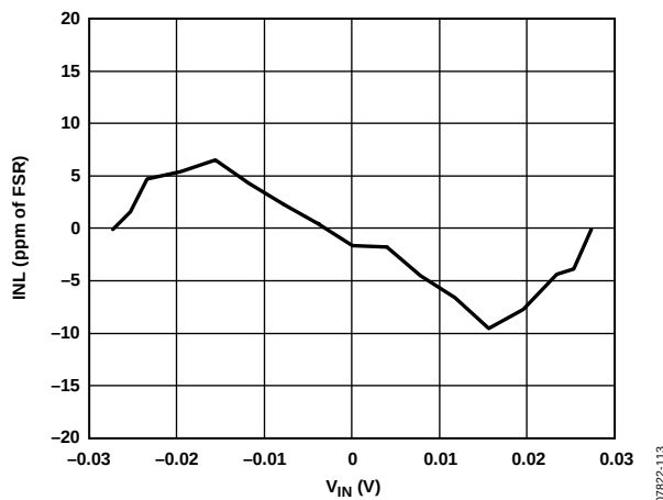
Figure 13. INL (Gain = 128)
