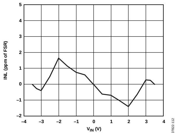
Figure 12. INL (Gain = 1)
