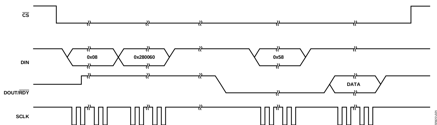
Figure 29. Single Conversion
