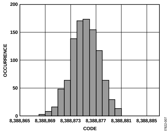
Figure 7. Noise Distribution Histogram ( V_{REF} = AV_{DD} = 5\text{ V} , Output Data Rate = 4.7 Hz, Gain = 128, Chop Disabled, Sinc 4 Filter)
