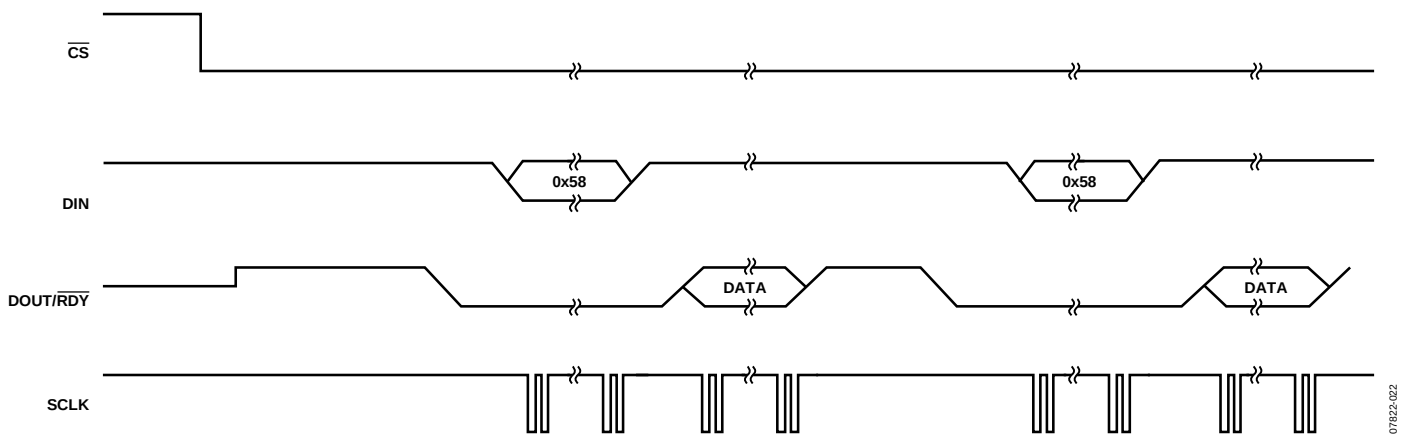
Figure 30. Continuous Conversion
