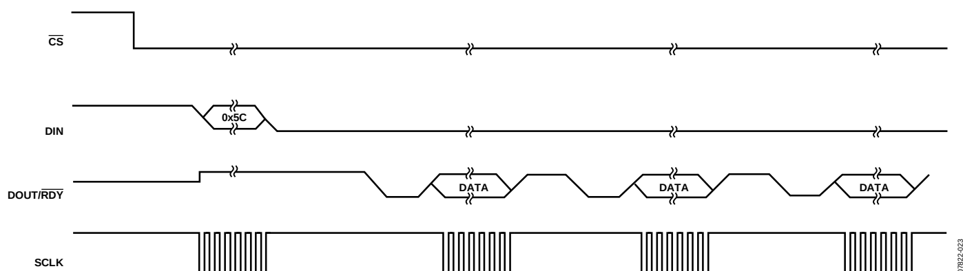
Figure 31. Continuous Read
