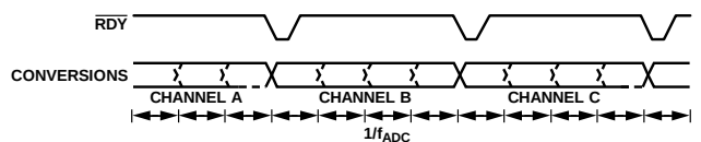
Figure 28. Channel Sequencer
