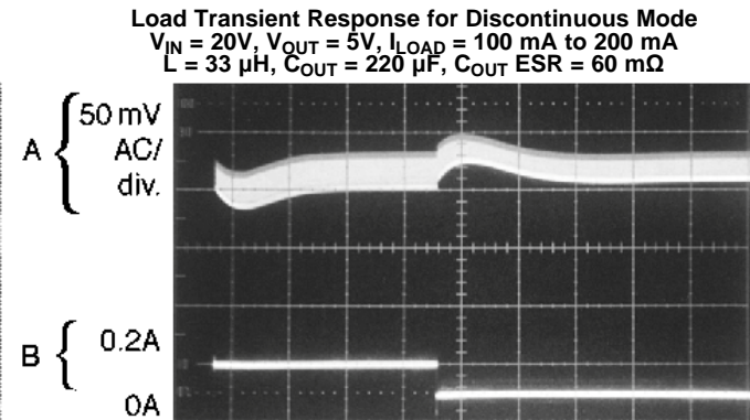
A: Output Voltage, 50 mV/div. (AC) B: 100 mA to 200 mA Load Pulse
