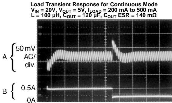
A: Output Voltage, 50 mV/div. (AC) B: 200 mA to 500 mA Load Pulse
