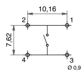
Non-illuminated
