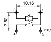
Bicolor - 2 LEDs
