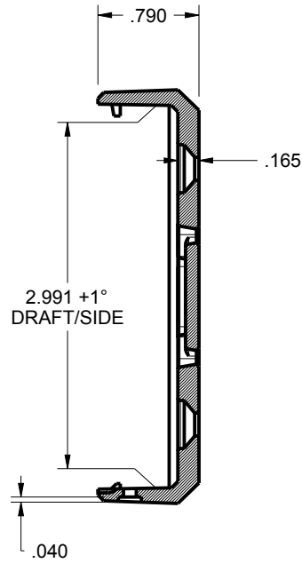
SECTION X-X
