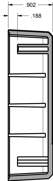
302112 TALL SECTION D-D SCALE 1.000
