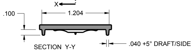
SECTION Y-Y
