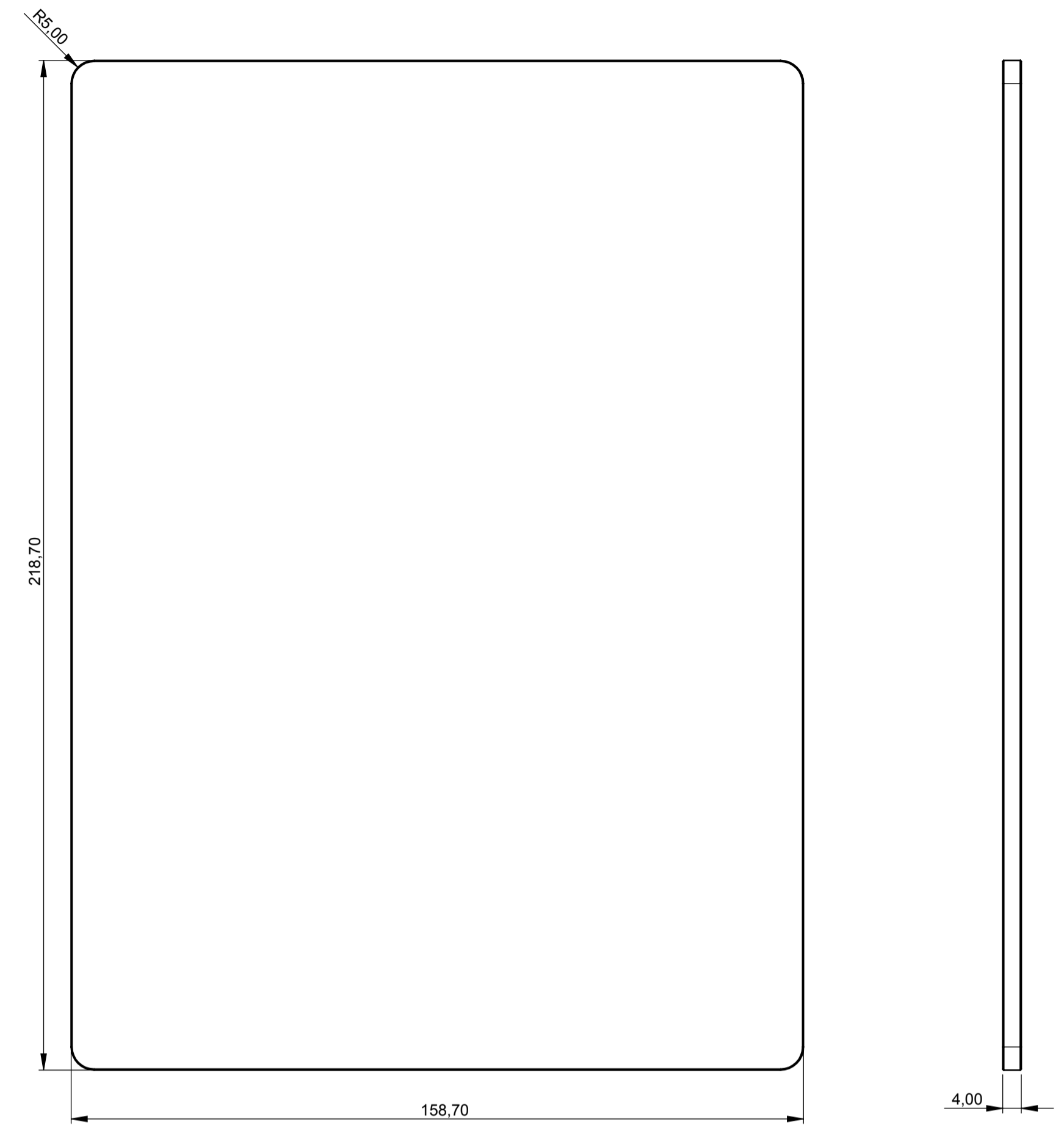
Glaspanel Glass panel
