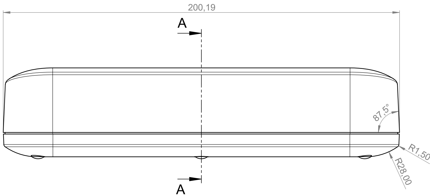
Ansicht "Z" View "Z"
